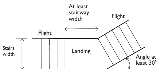
Diagram 3 Change of direction in places of assembly Par. 1.1.12
