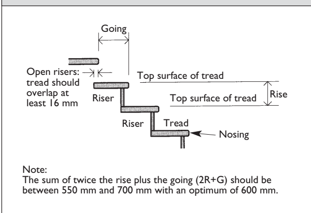
Diagram 1 Measuring rise and going Par. 1.1.4
